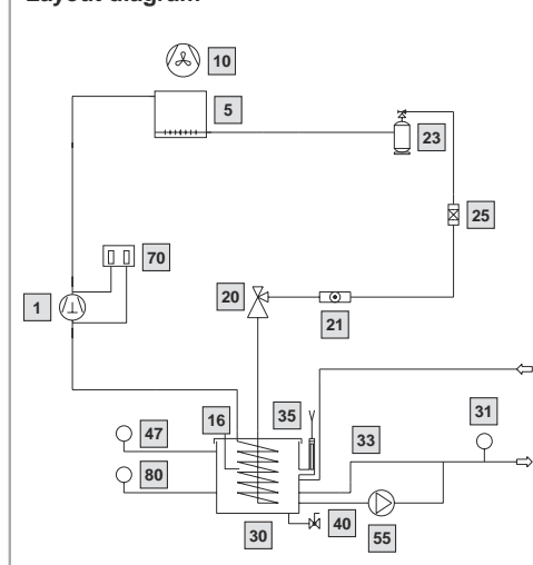
Layout diagram
